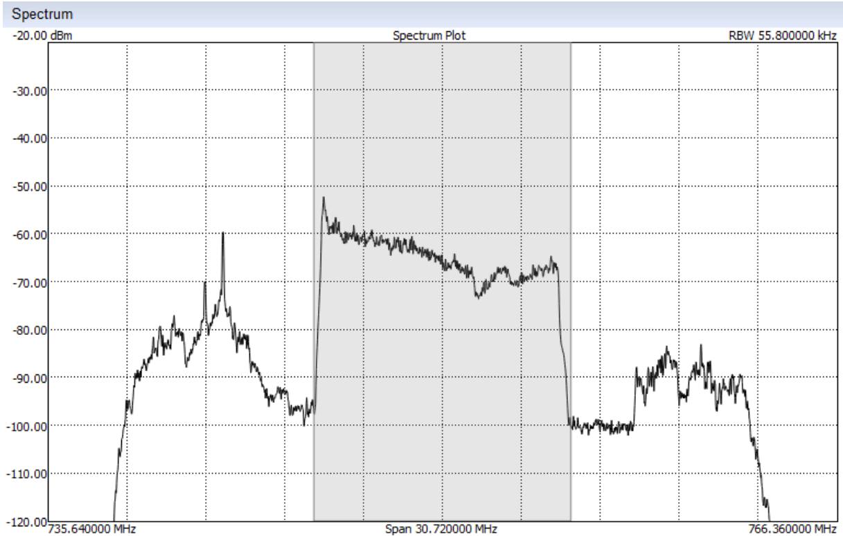
Figure 58: LTE spectrum plot showing a cell signal.
