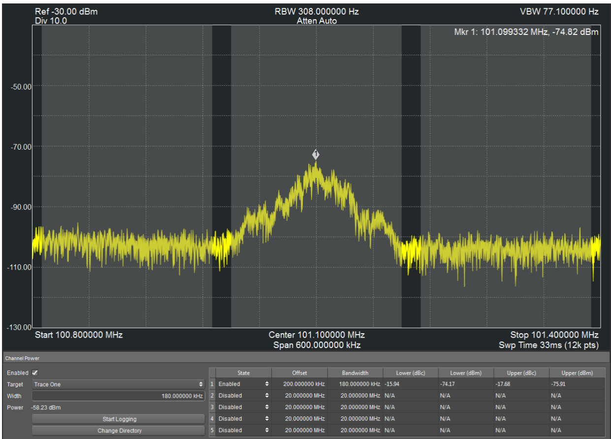
Figure 66: Channel Power on a Broadcast FM Signal
