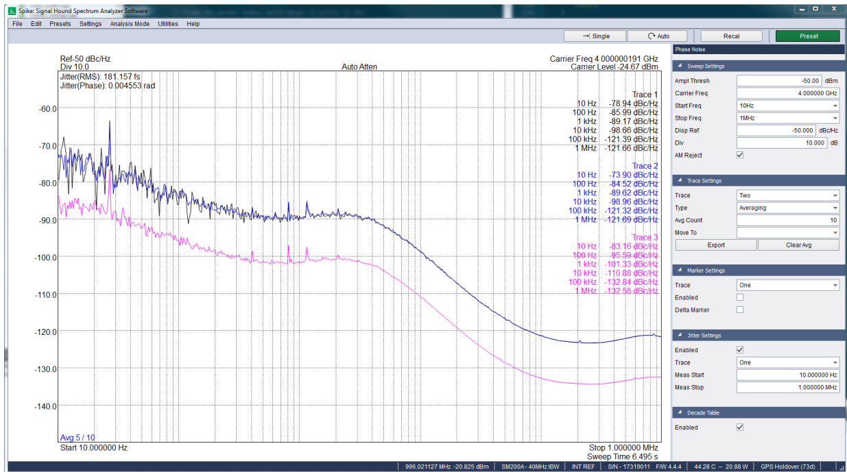
Figure 18: SM200A measuring the phase noise of a signal generator at 1 and 4 GHz carriers.
