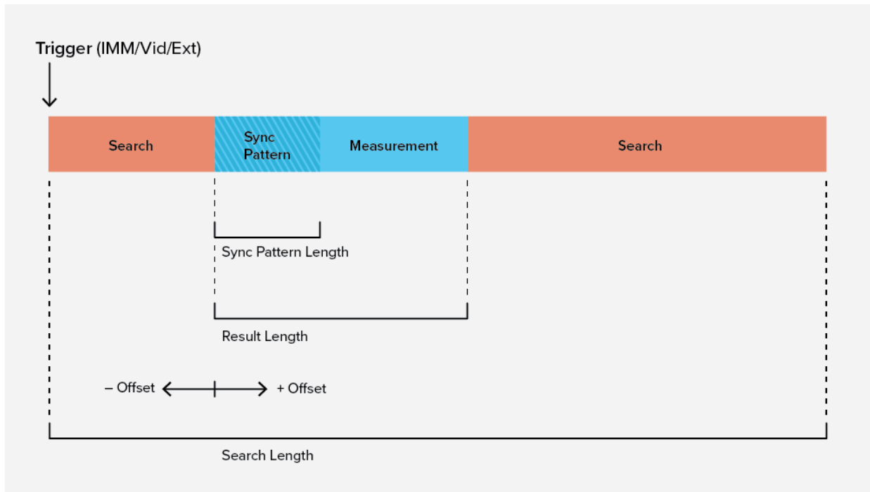
Figure 20: This diagram illustrates how sync search is performed and how the measurement is framed within the search length.
