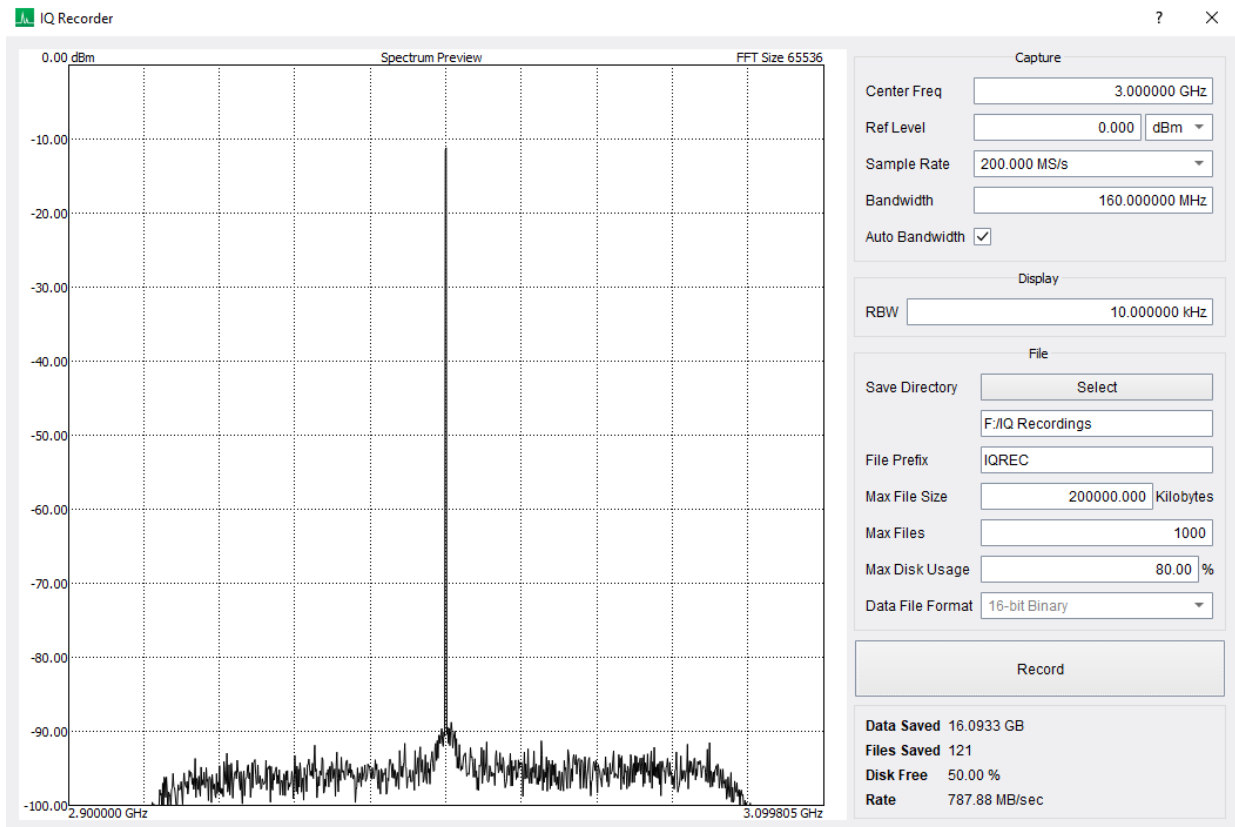
Figure 64: I/Q Recorder Utility.
