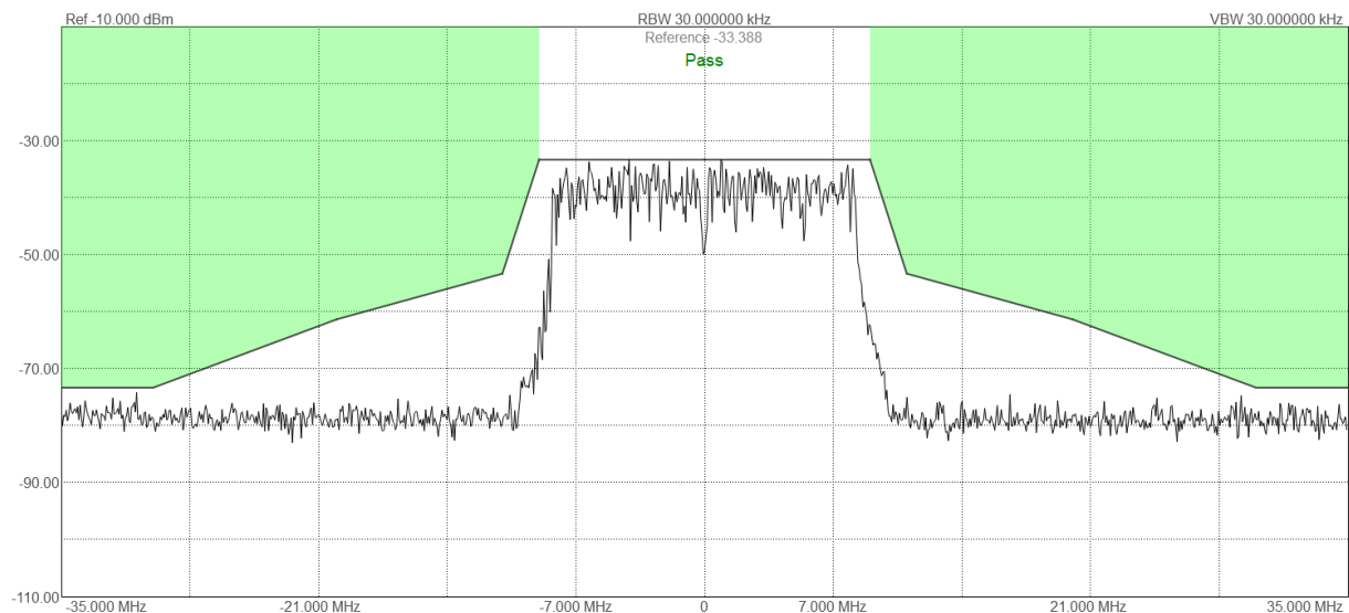
Figure 47: Testing input against an 802.11 OFDM transmission mask.
