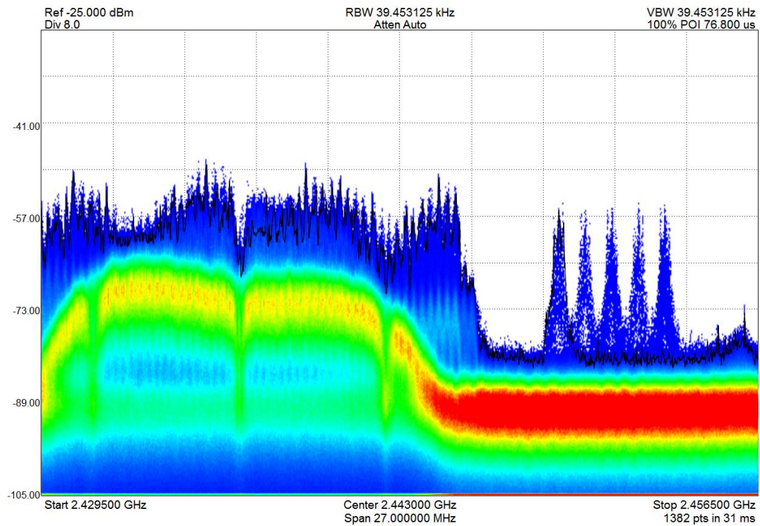
Figure 92: Real-time persistence display of a wireless router and Bluetooth® headset coexisting in the ISM band.
