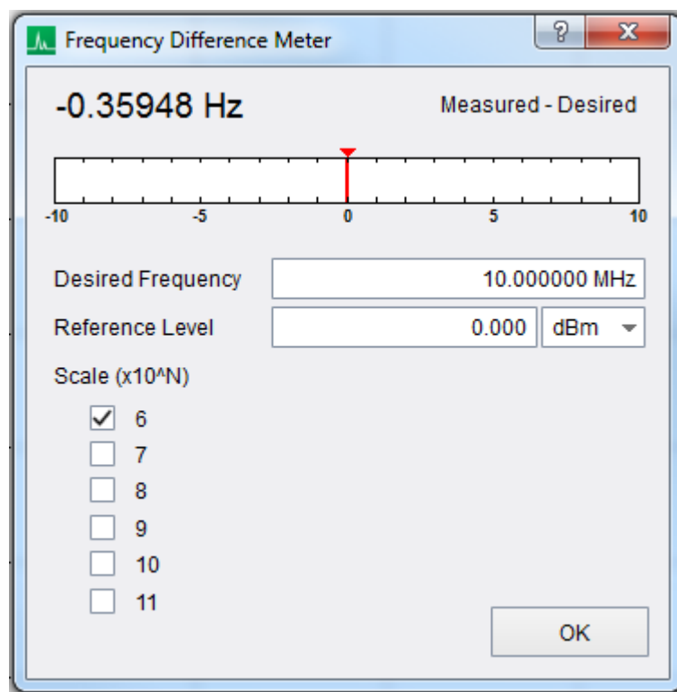
Figure 76: Frequency difference meter observing frequency difference between two 10MHz oscillators
