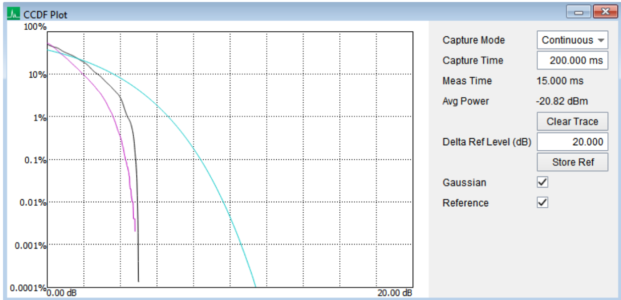
Figure 11: Comparing synthetic noise signal to a Gaussian reference and ideal test signal.
