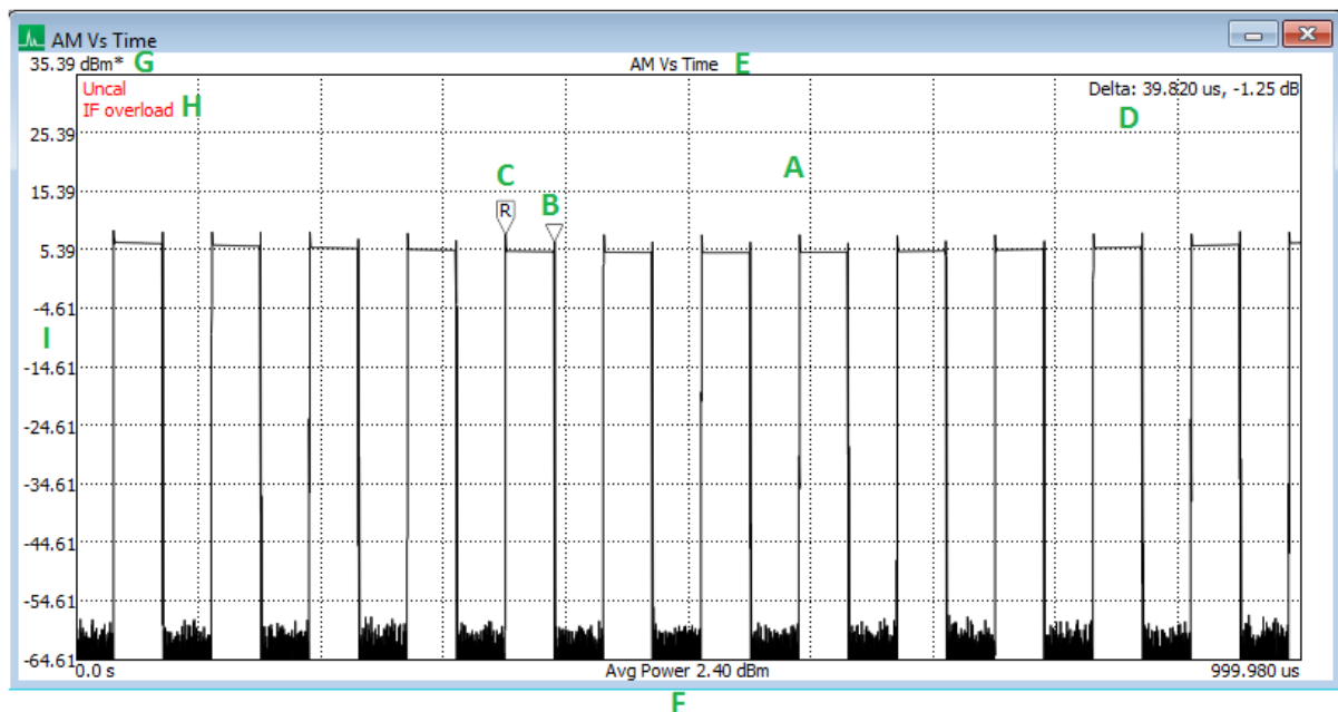
Figure 87: Basic plot areas of interest.
