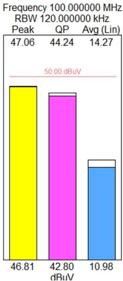
Figure 30: Bar Meters Measuring Pulsed Signal
