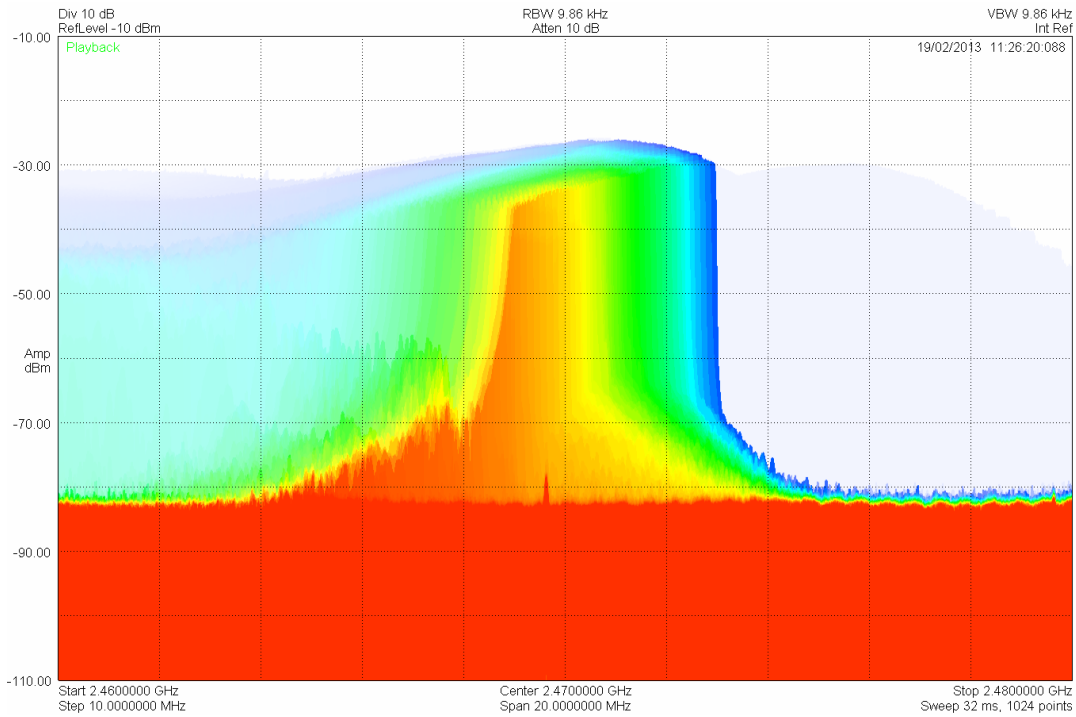
Figure 91: Sweep mode persistence showing the signal from a poorly shielded commercial microwave oven.
