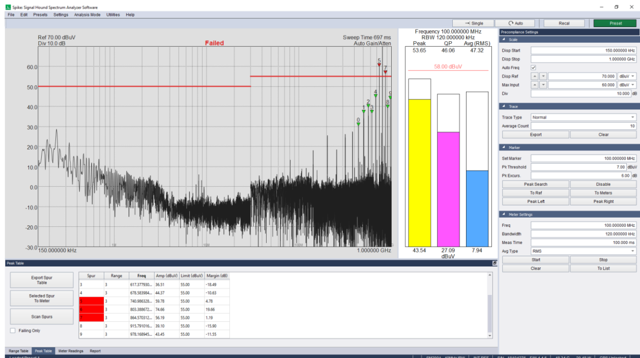
Figure 26: Radiated Emissions Precompliance Testing for the VSG25A
