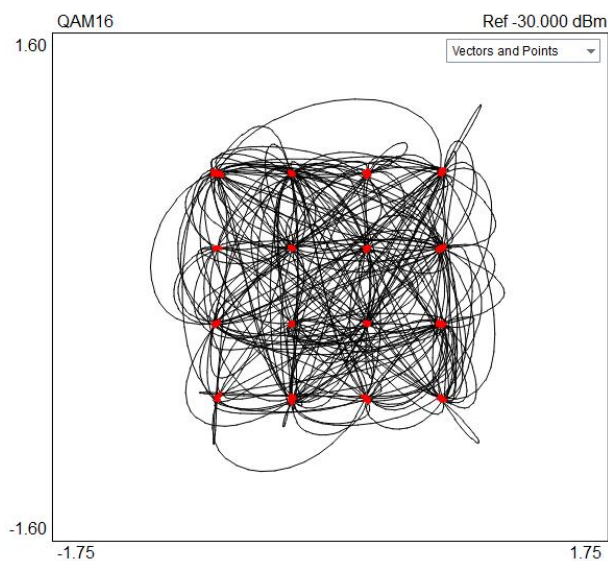
Figure 23: Constellation Diagram for a QAM 16 Input Signal
