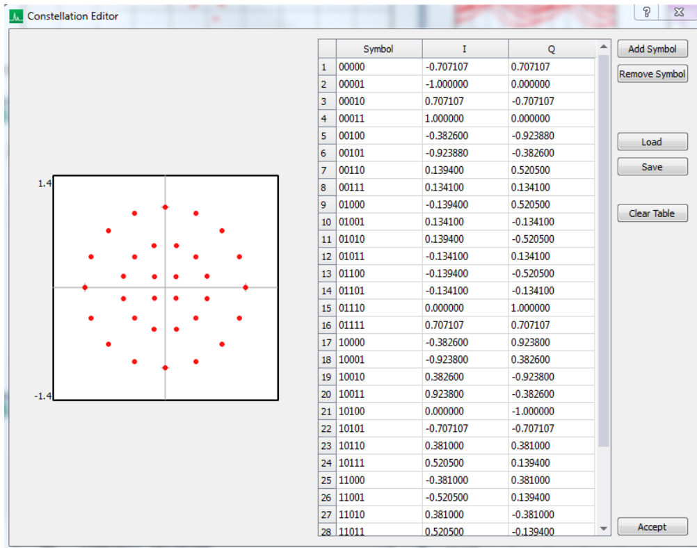
Figure 19: APSK32 in the constellation editor.
