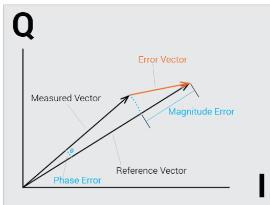
Figure 22: Visualization of the EVM, Magnitude and Phase Error Calculations
