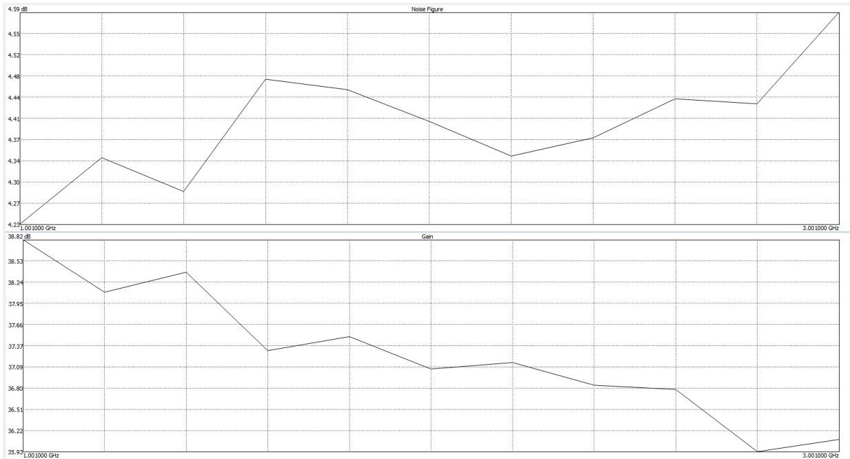
Figure 50: Noise figure and gain plots of a small wideband amplifier, tested with an SM200A and an Agilent 346B noise source.
