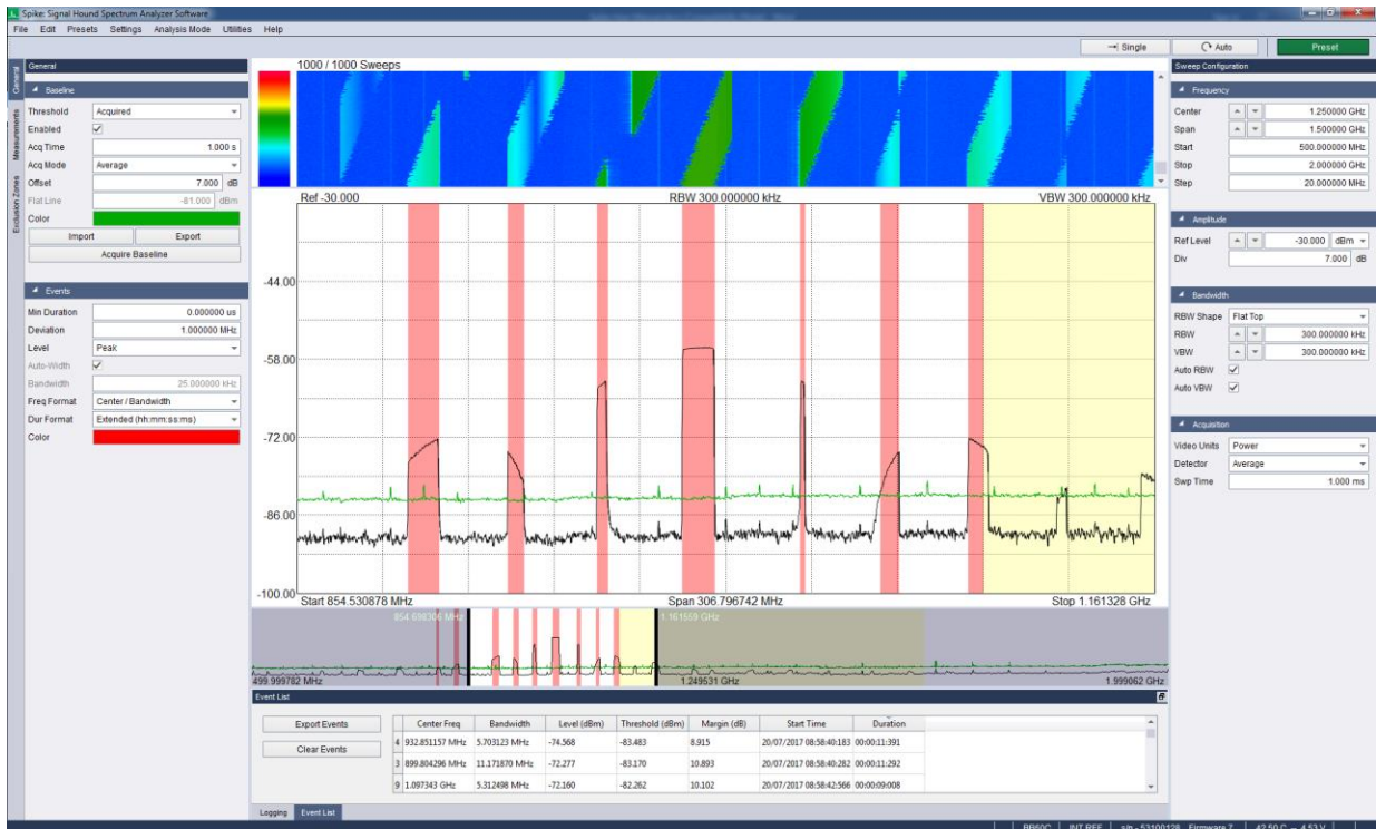
Figure 34: Detecting events in Interference Hunting mode with an acquired baseline. Yellow area on right is an exclusion zone.
