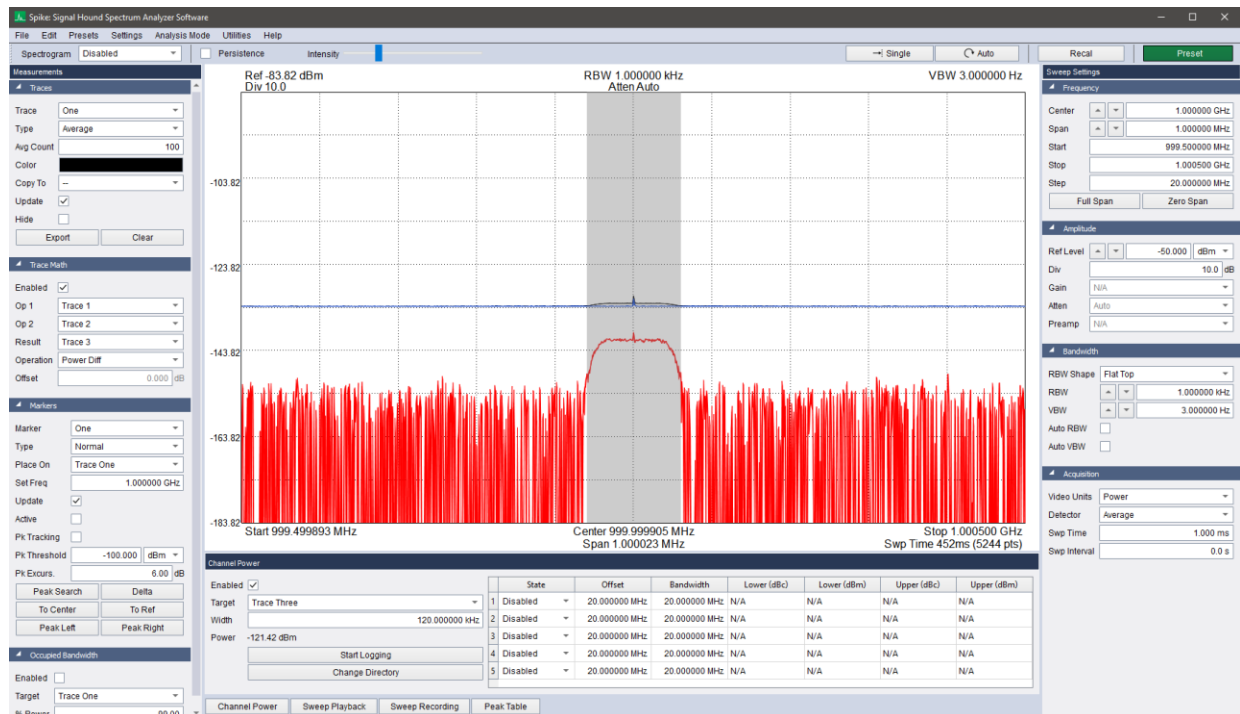
Figure 68: Power difference function measuring signal power below the instrument noise floor.
