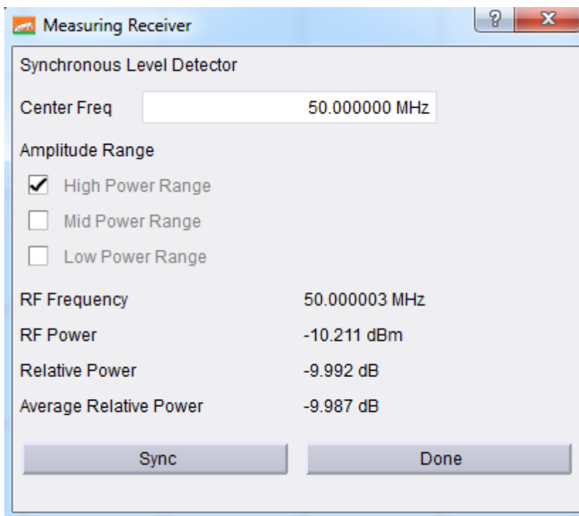
Figure 69: Measuring Receiver Control Dialog
